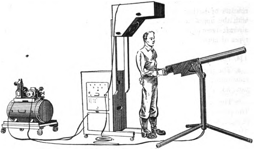
Figure 93. Antiaircraft machine gun trainer, M9.
