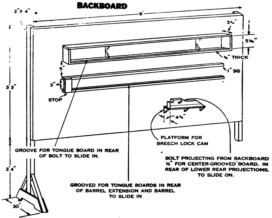
Figure 145. Construction of backboard for recoiling parts.
