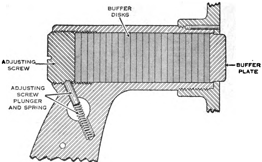
Figure 23. Shock-absorbing group.
