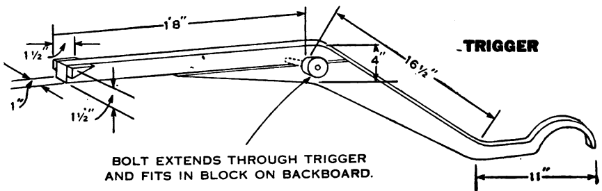
Figure 143. Construction of the trigger.
