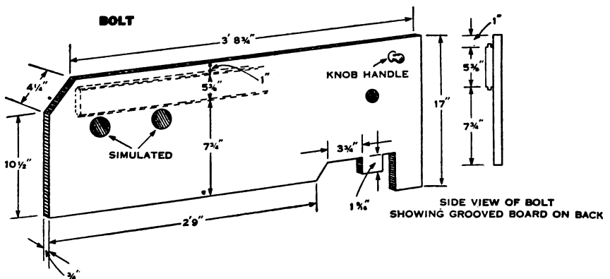
Figure 146. Construction of bolt.
