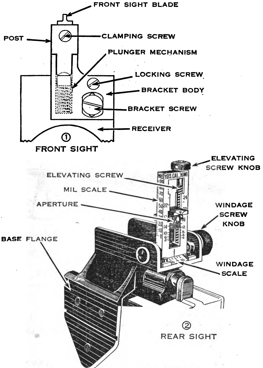
Figure 4. Sights of the M1919A4 and M1919A6 gun.
