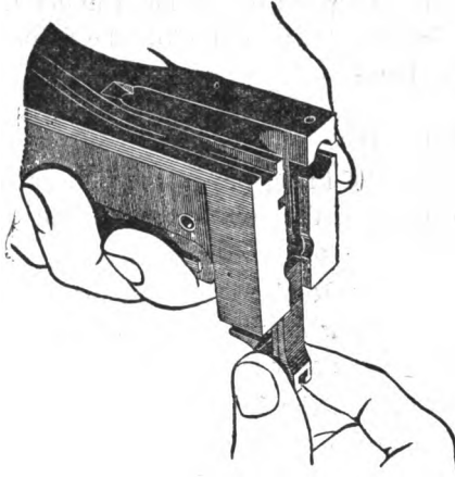
Figure 16. Removing the sear.
