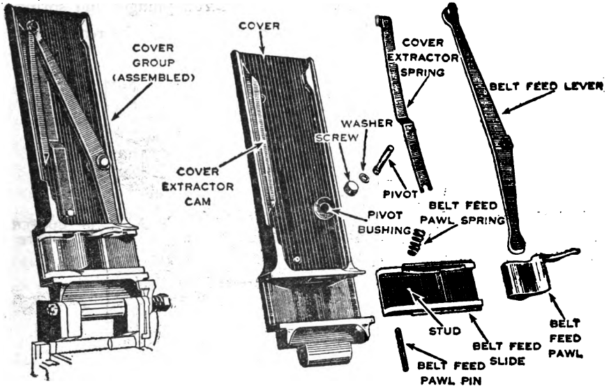
Figure 22. Cover group.
