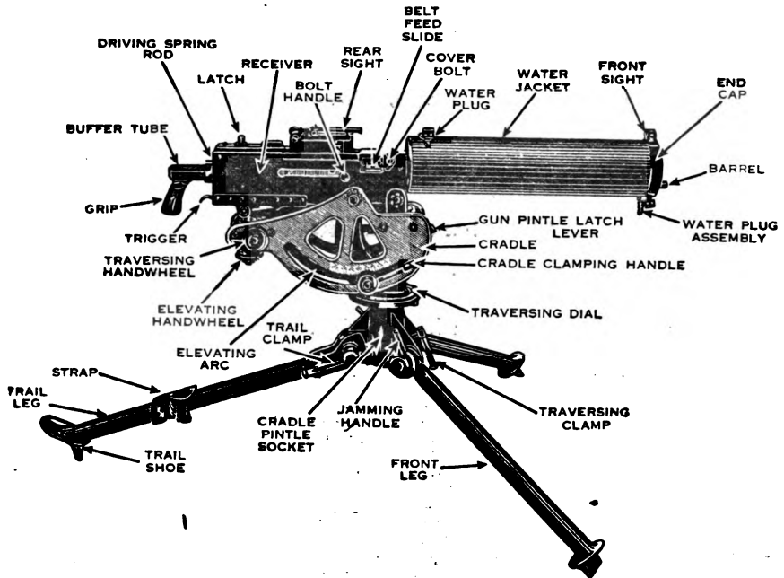
Figure 1. Browning machine gun, caliber .30, M1917A1.
